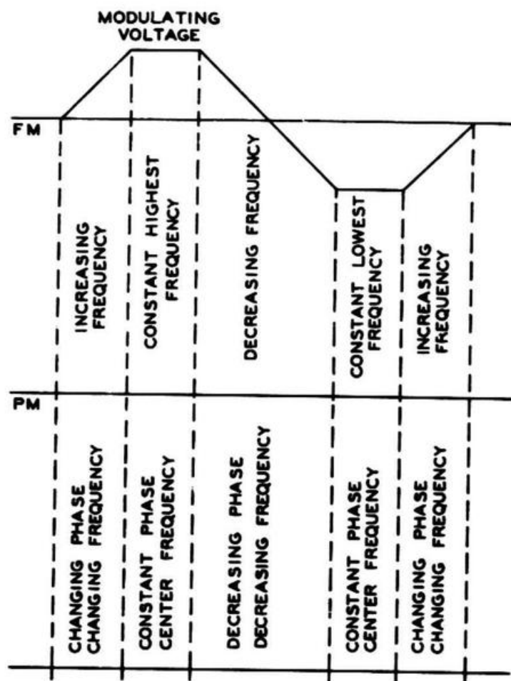
Figure 4-13. Comparison of FM and PM
