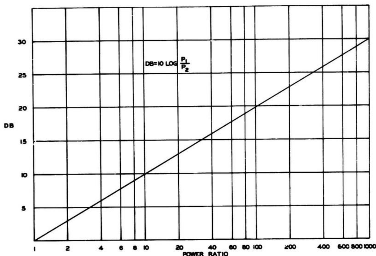
Figure 1-1. Relationship Between Power Ratio and Decibels
