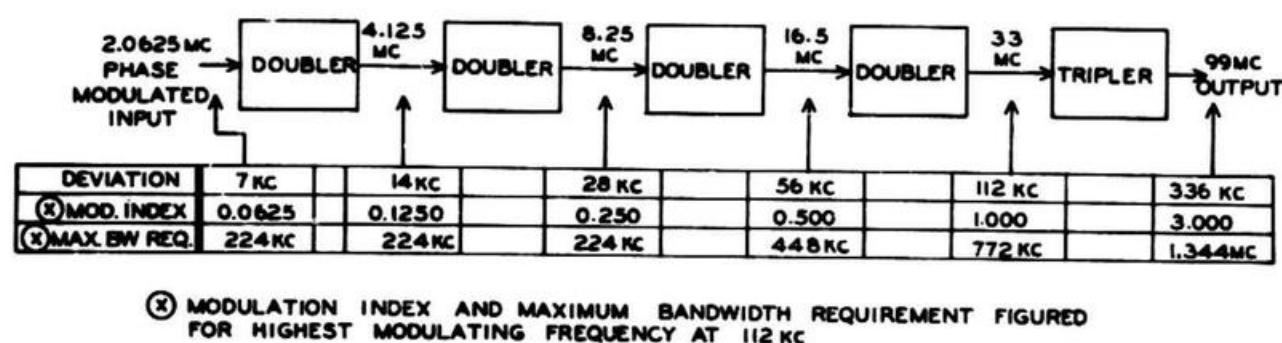
Figure 6-14. Typical Multiplier Arrangement for Exciter
