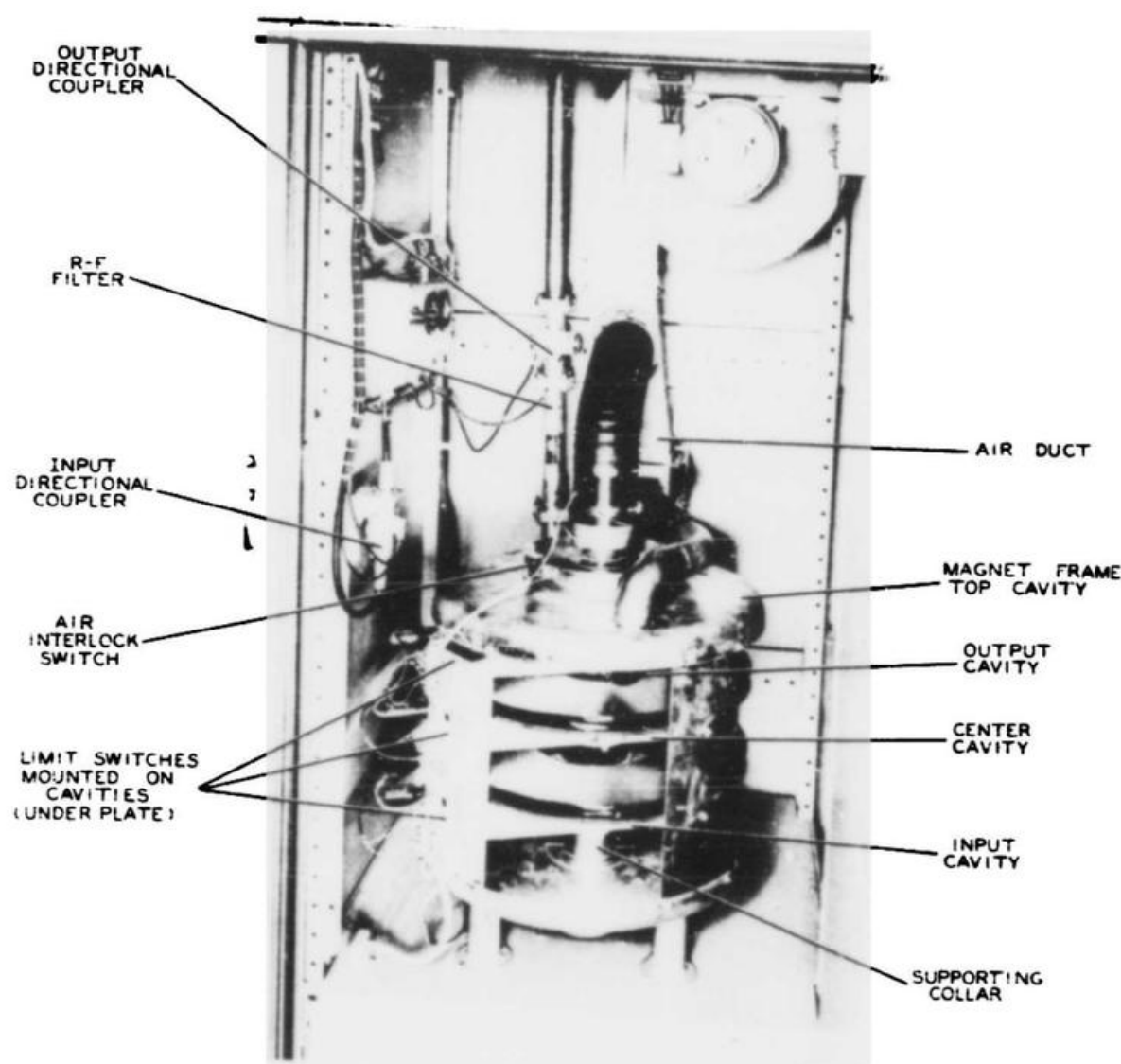
Figure 7-1a. Typical Klystron Amplifier Assembly (1000 mc)
