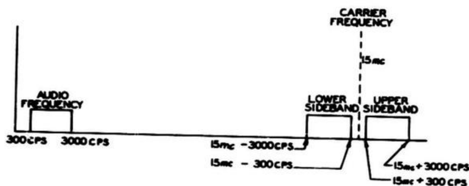
Figure 4-4. Location of Sidebands with Voice Modulation
