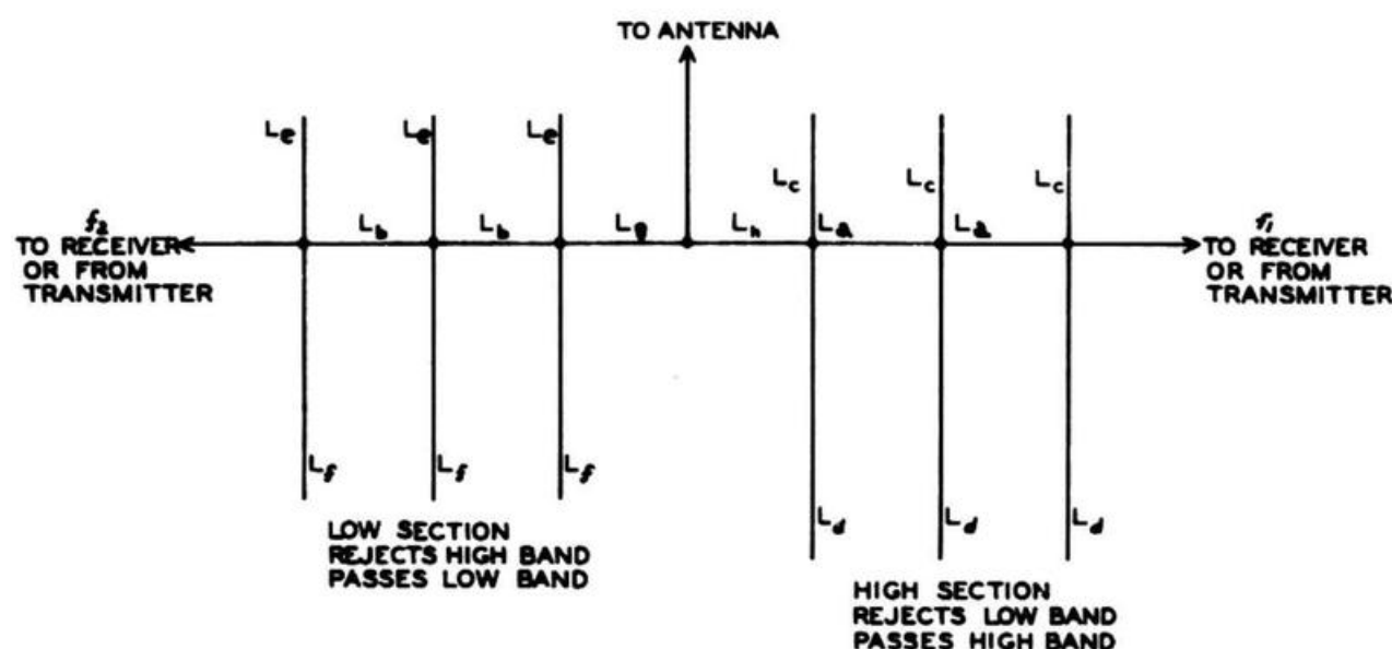
Figure 9-29. Schematic Diagram of Coaxial Diplexing Filter
