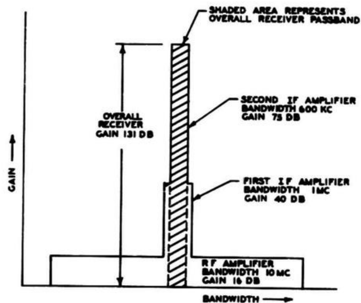
Figure 8-8. Typical Receiver Bandwidth and Gain Relationships
