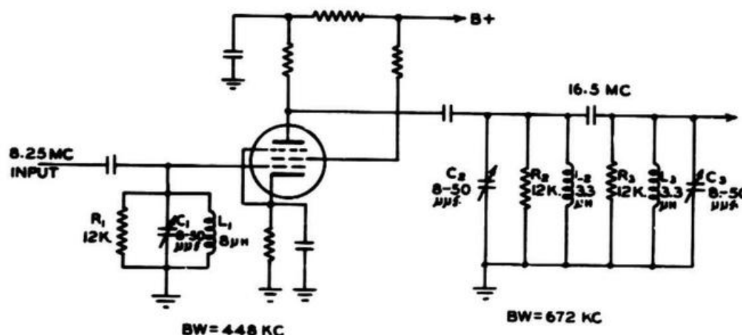
Figure 6-13. Doubler Circuit
