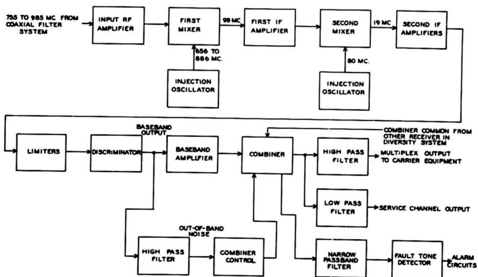
Figure 8-1. Block Diagram of Tropospheric Scatter FM Receivers
