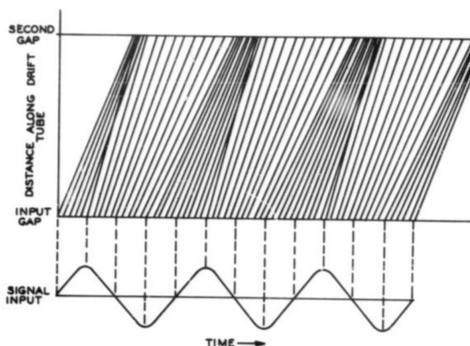
Figure 7-5. Mechanics of Velocity Modulation
