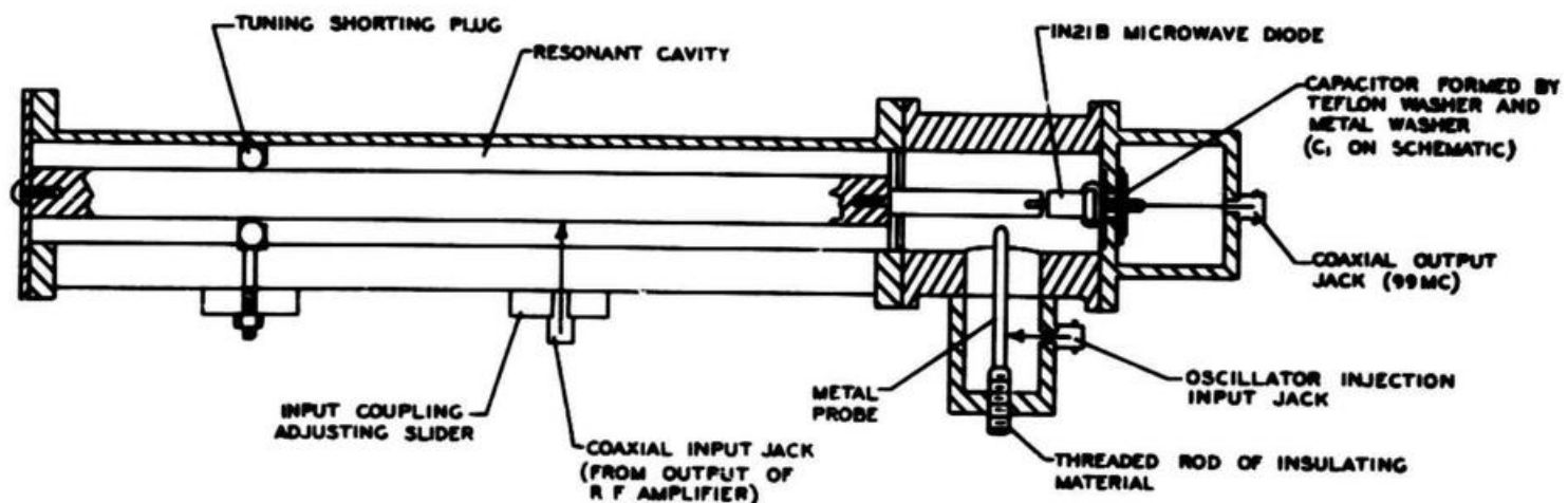
Figure 8-6. Cross Sectional View of Crystal Mixer Assembly
