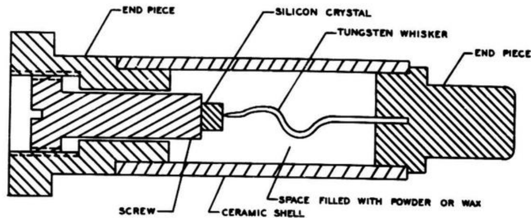
Figure 8-5. Cross Section of a Crystal Cartridge
