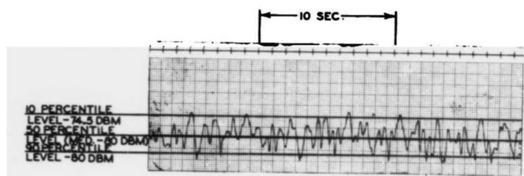
Figure 3-12. Typical Signal Level Recording Showing Short-Term Fading
