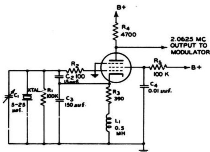
Figure 6-10. Crystal-Controlled Oscillator Used to Provide Modulator Input
