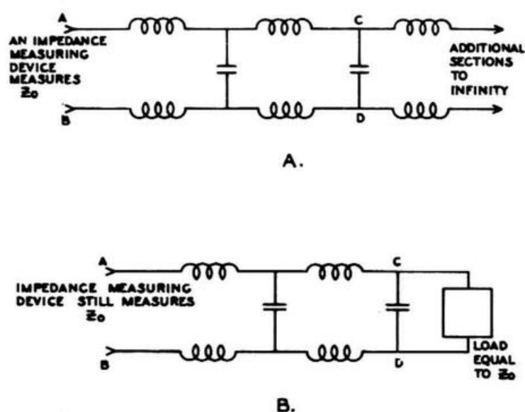
Figure 9-2. Development of Characteristic Impedance
