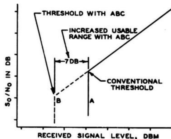
Figure 8-21. S/N Ratio as a Function of Received Signal Level for an FM Receiver with and without Automatic Bandwidth Control Circuit
