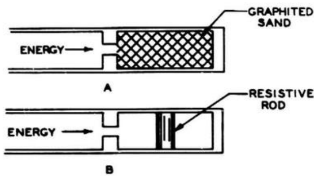
Figure 9-27. Terminations for Minimum Reflection
