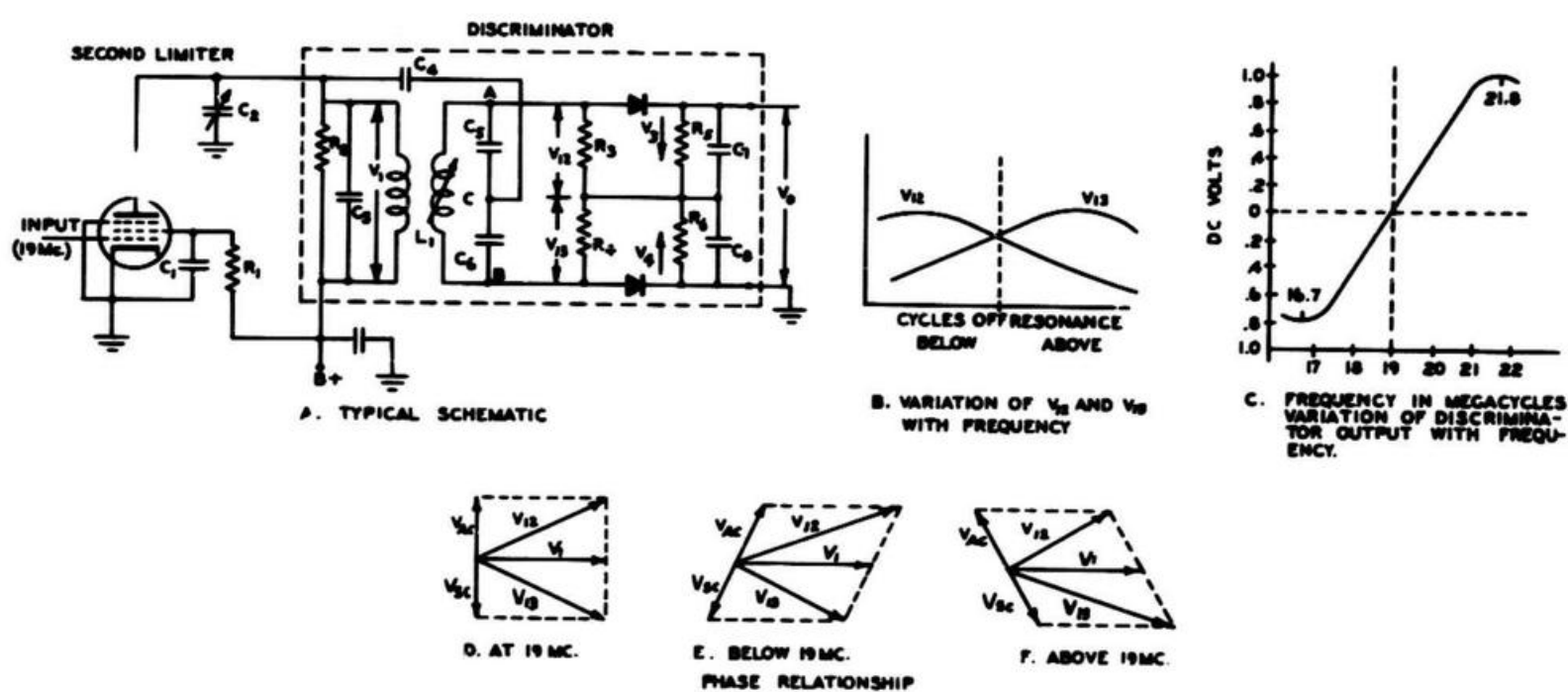
Figure 8-16. Operation of Foster-Seeley Discriminator
