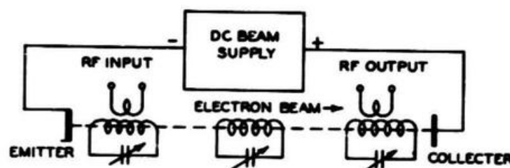
Figure 7-4. Representation of Klystron Operation
