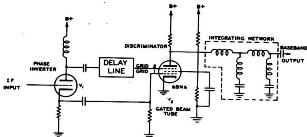
Figure 8-17. Pulse Counter Discriminator Circuit
