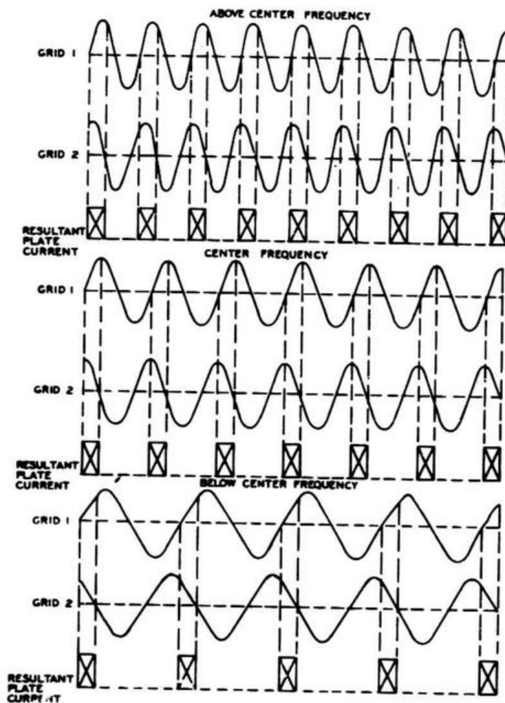
Figure 8-18. Relationship of Signal in Pulse Counter Discriminator
