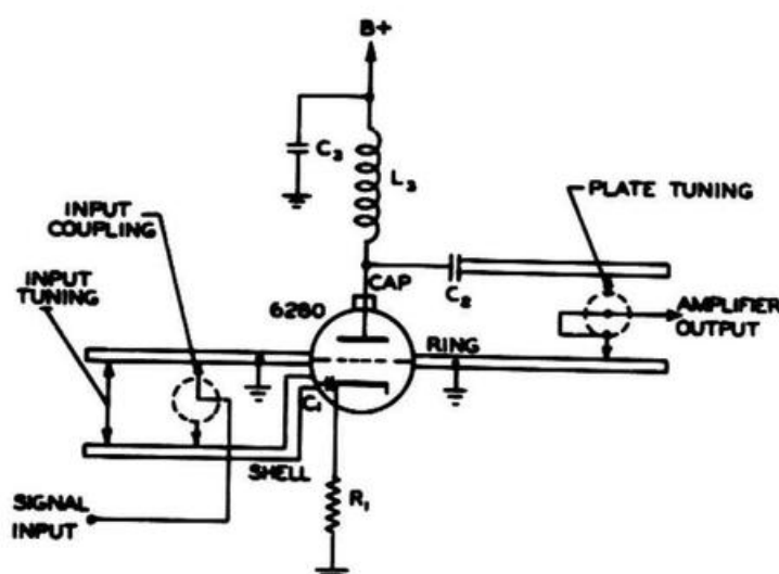
Figure 8-3. Schematic Diagram of R-F Amplifier
