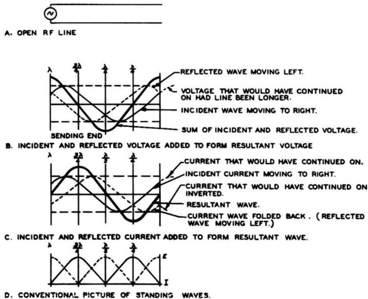
Figure 9-4. Formation of Standing Waves in Open Line
