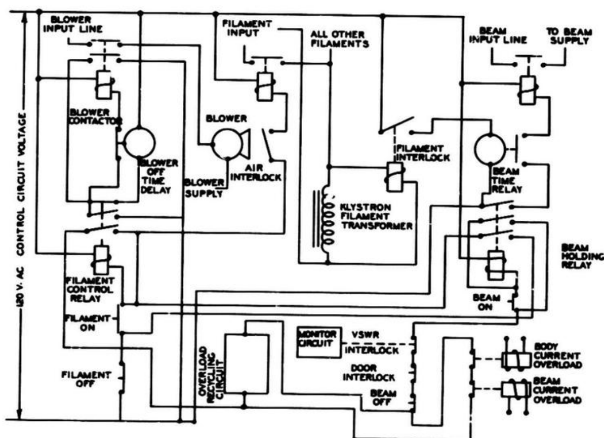
Figure 7-7. Typical Power Amplifier Control Circuit
