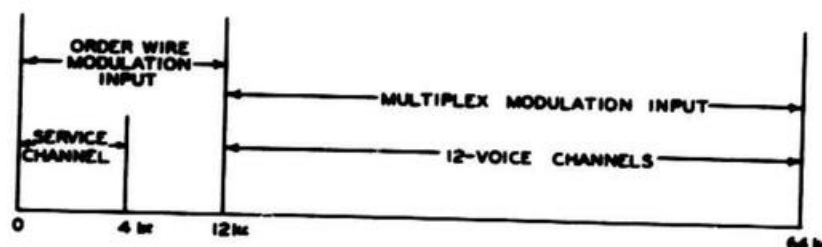
Figure 3-20. Typical Baseband Spectrum for 12-Channel System
