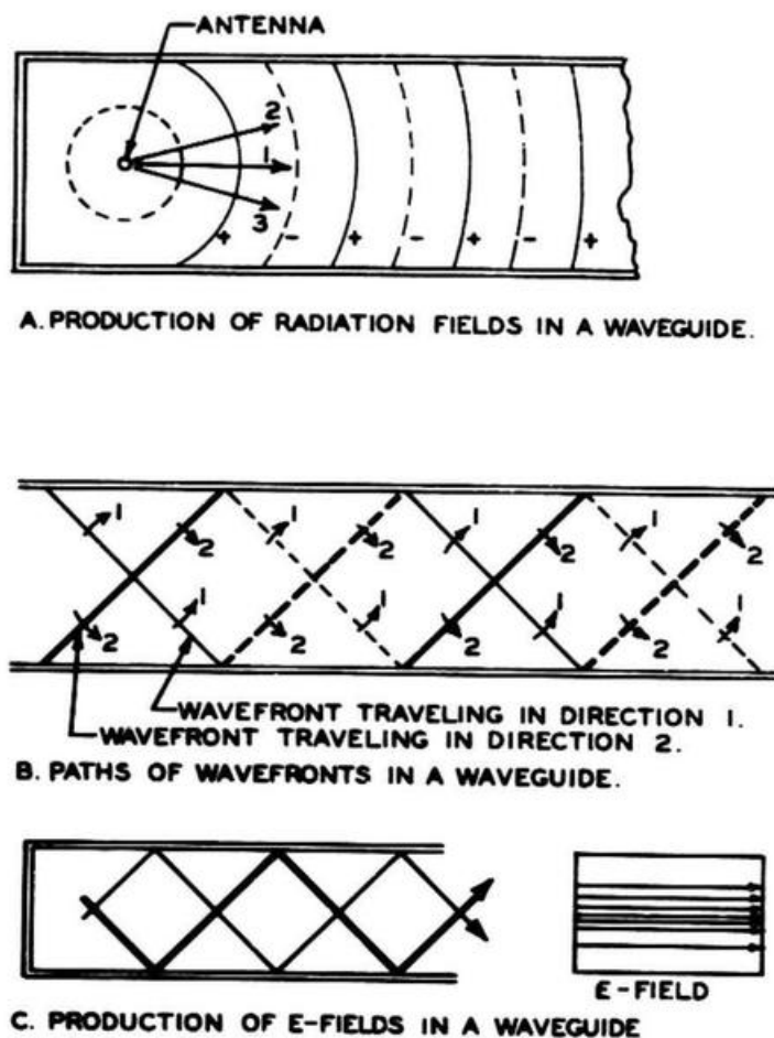
Figure 9-16. Propagation of Radio Waves in Wave Guides
