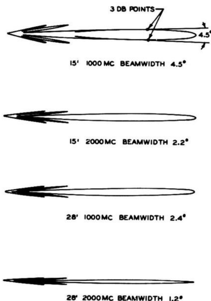
Figure 9-36. Typical Radiation Patterns for Parabolic Antenna Systems
