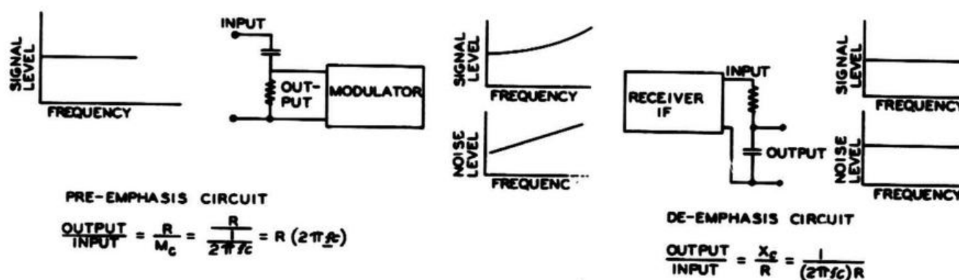
Figure 5-6. Pre-Emphasis and De-Emphasis Circuits
