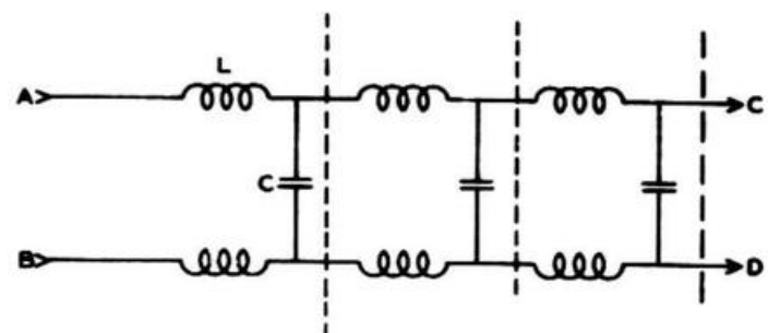
Figure 9-1. Approximate Representation of R-F Transmission Line
