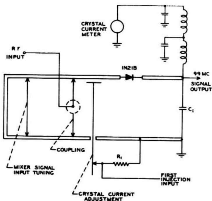
Figure 8-7. Schematic Diagram of Crystal Mixer Assembly
