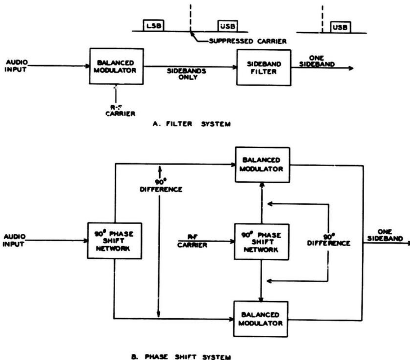
Figure 4-7. Two Systems for Generating Single-Sideband Signals
