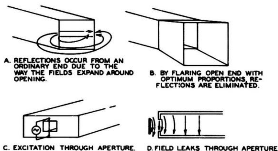
Figure 9-22. Excitation with Electromagnetic Fields
