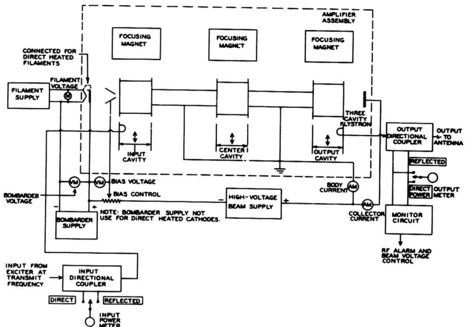
Figure 7-6. Power Supplies and Metering Circuits
