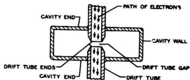
Figure 7-3. Klystron Cavity Assembly, Simplified Sectional View
