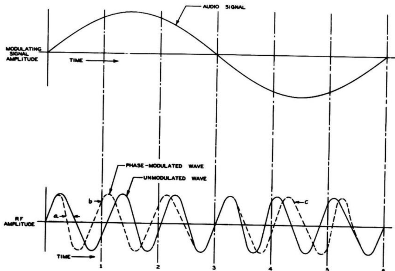
Figure 4-12. Representation of Phase Modulation
