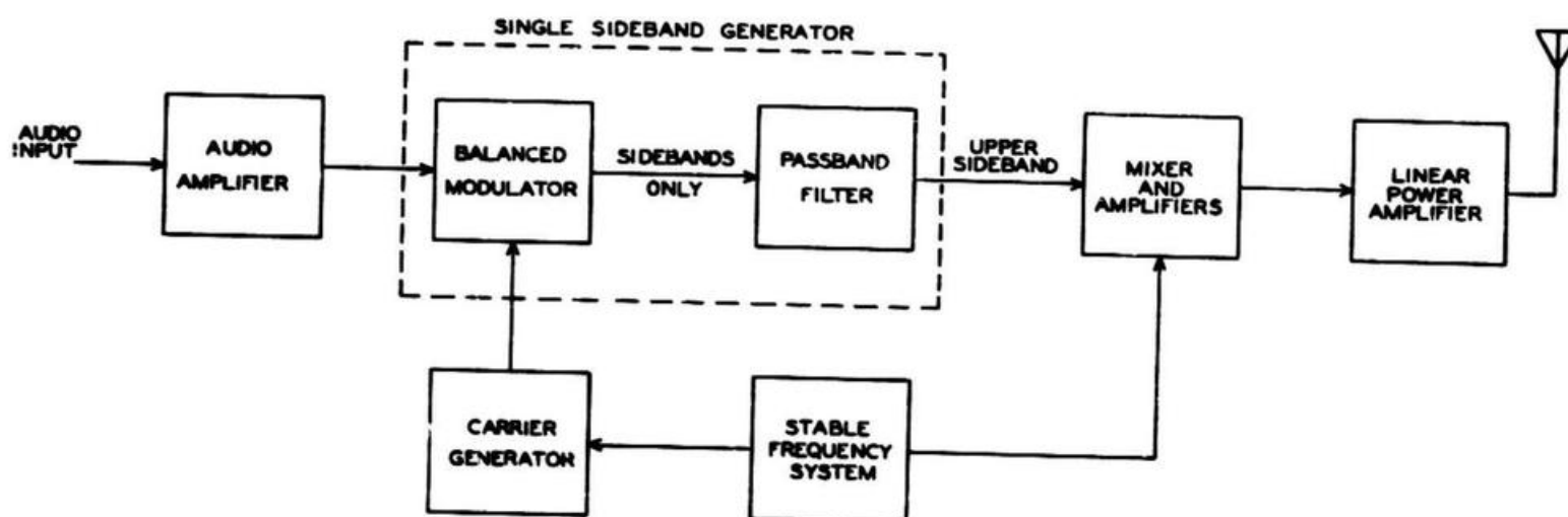
Figure 4-5. Single-Sideband Transmitting System
