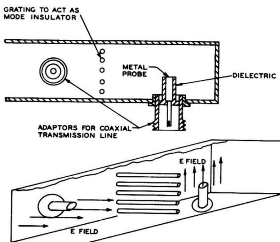
Figure 9-34. Bipolarized Feed System
