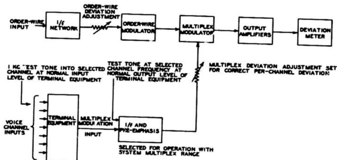
Figure 6-22. Deviation Adjustments
