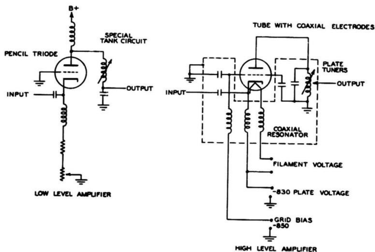
Figure 6-20. Two Typical Output Amplifier Circuits
