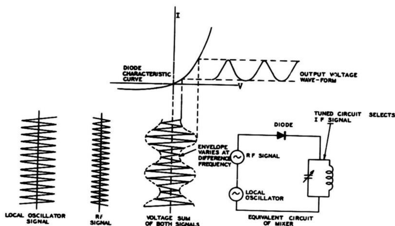
Figure 8-4. Mixer Action and Equivalent Circuit
