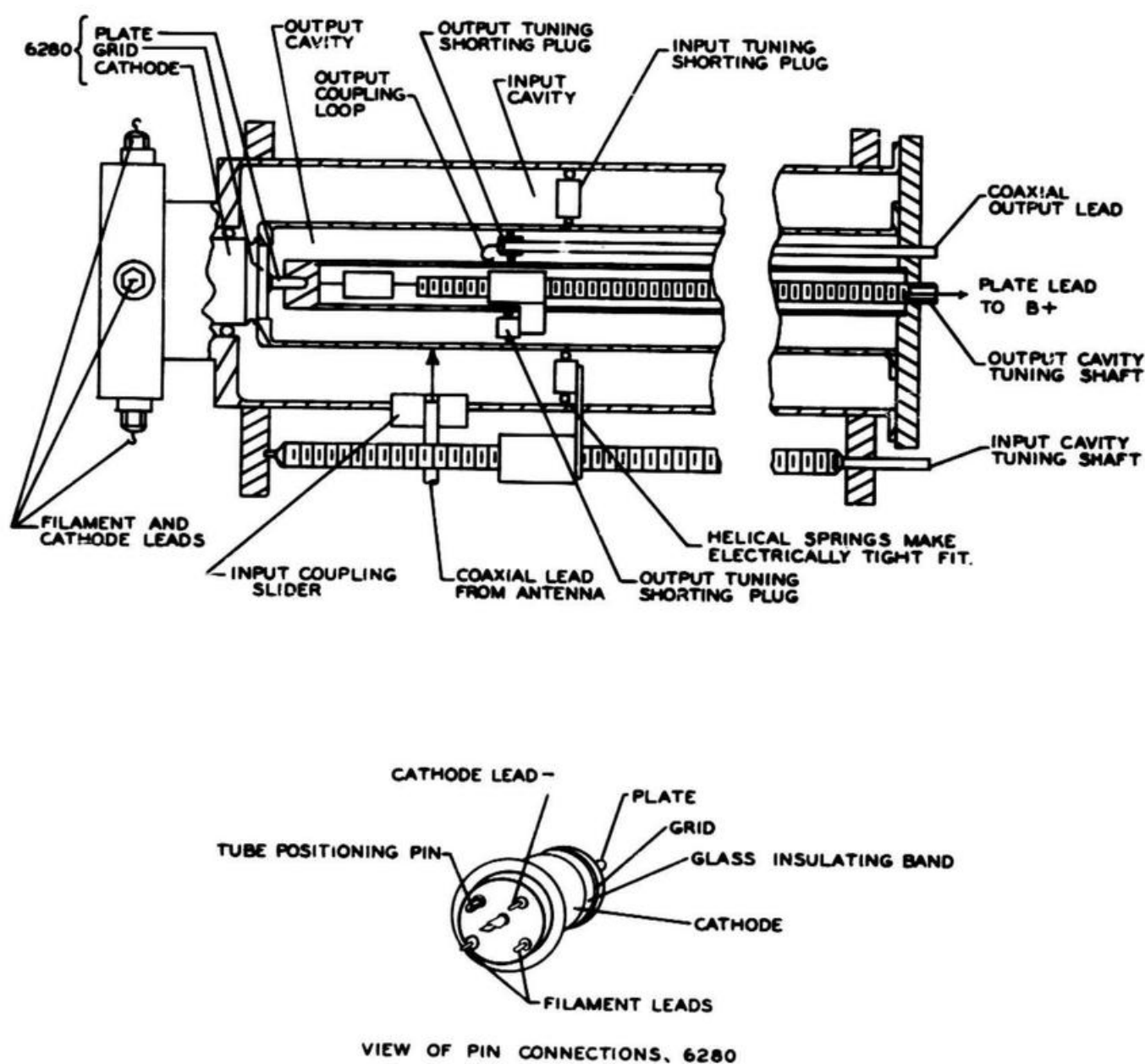
Figure 8-2. Cross Sectional View of R-F Amplifier Assembly
