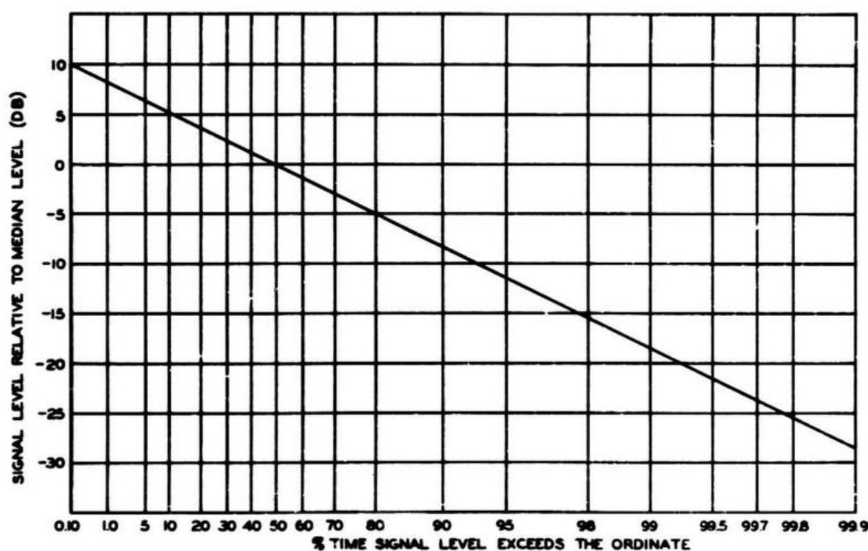
Figure 3-11. Short-Term Fading Characteristics
