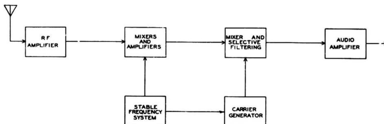
Figure 4-8. Single-Sideband Receiving System
