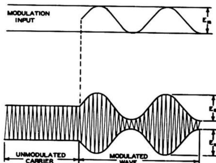
Figure 4-2. Amplitude Modulation
