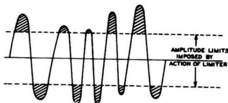
Figure 8-12. Limiter Action on Frequency-Modulated Wave
