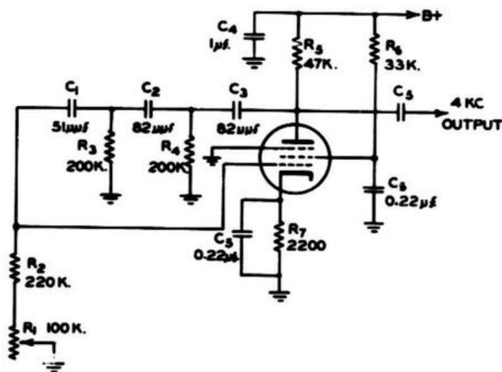
Figure 6-12. Typical Phase-Shift Oscillator
