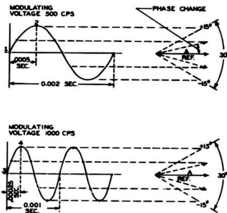
Figure 4-14. Vector Representation of Phase Modulation
