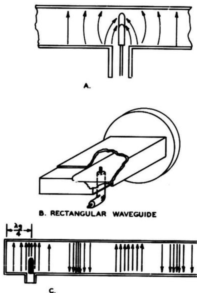
Figure 9-20. Exciting Wave Guide with Electric Field
