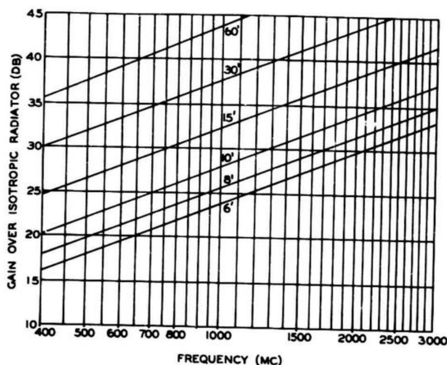
Figure 9-37. Parabolic Antenna Gain Curves
