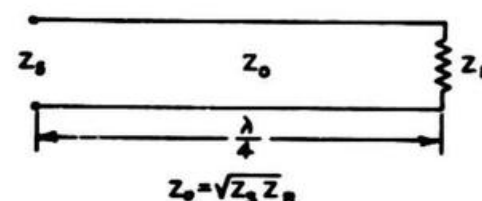
Figure 9-11. Quarter-Wave Line Section as Impedance Transformer
