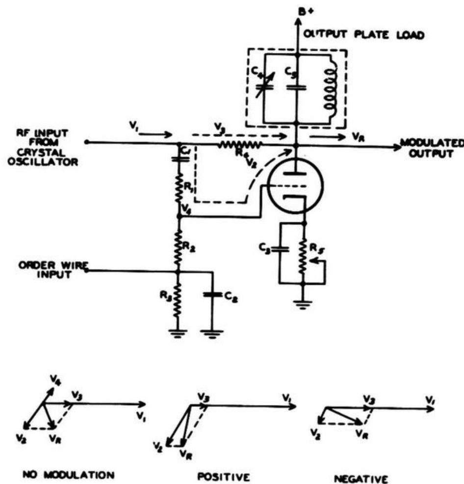
Figure 6-5. Typical Order Wire Modulator Circuit
