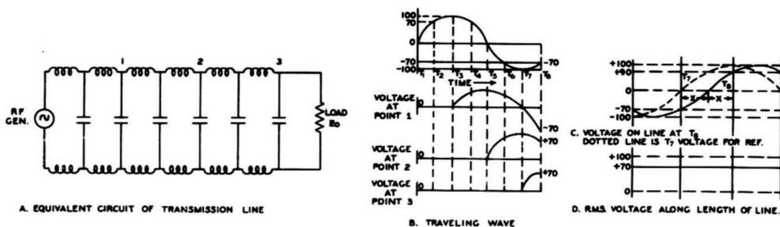
Figure 9-3. Wave Motion on Matched Transmission Line
