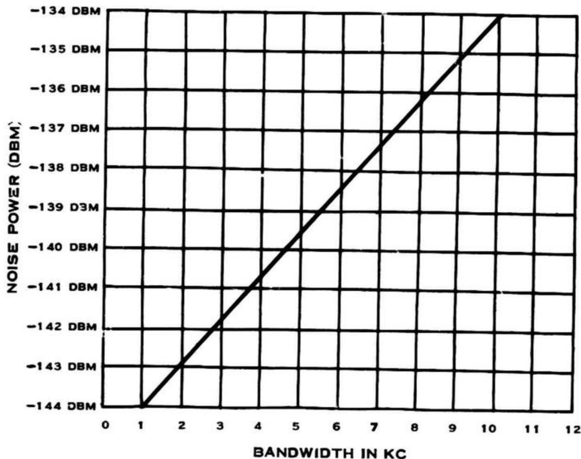
Figure 5-2. Change in Noise Power with Bandwidth
