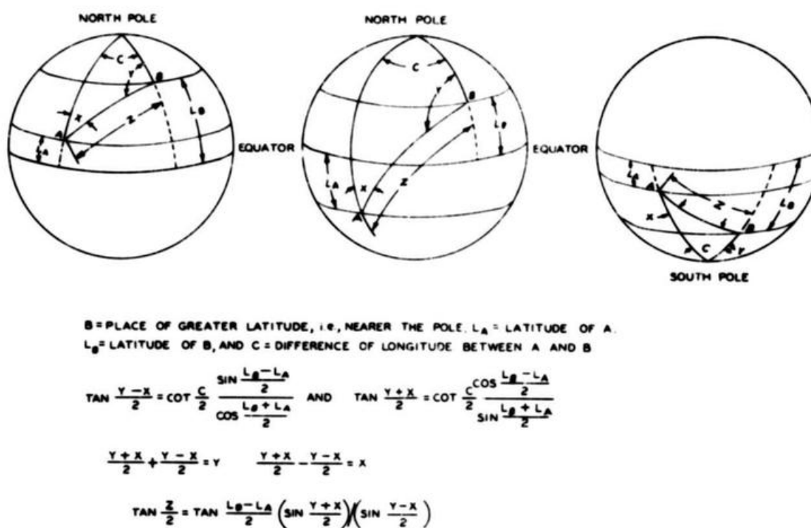
Figure 10-1. Calculations for Determining Great-Circle Path Length and Bearing
