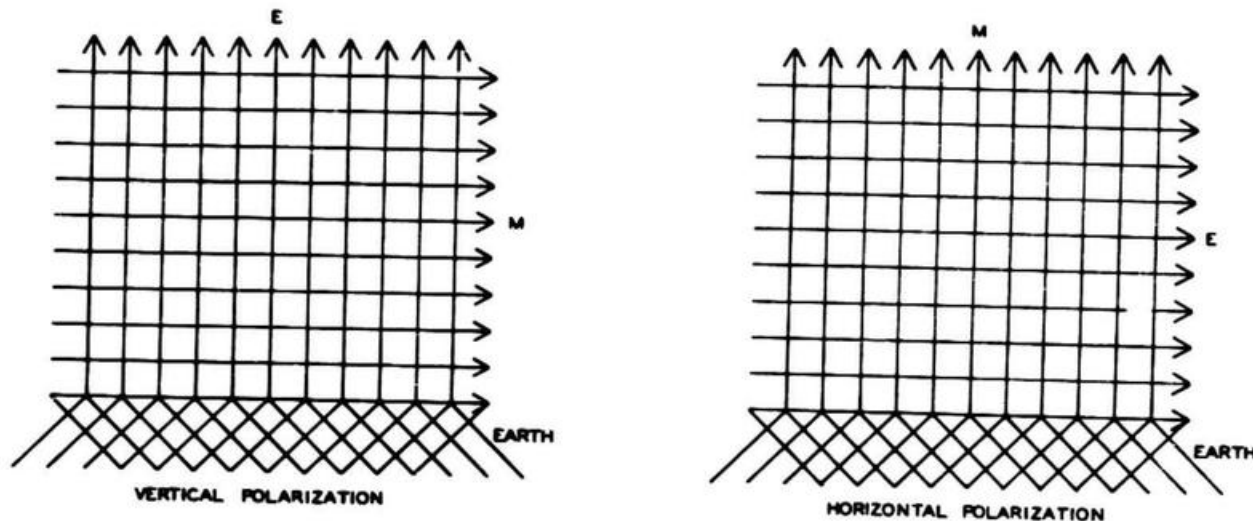
Figure 2-1. Representation of Magnetic and Electric Fields in Wave Front
