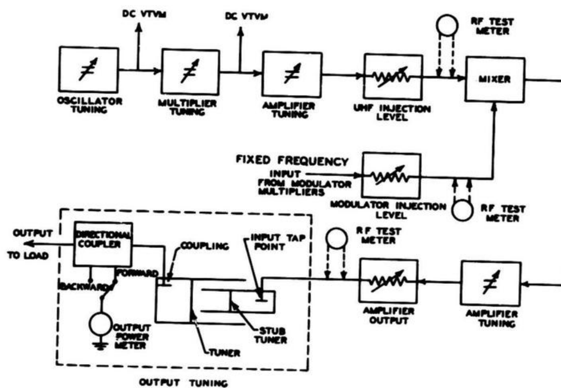
Figure 6-21. Typical Exciter Tuning Adjustment
