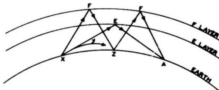
Figure 2-6. Multipath Transmission Which Could Result in Fading
