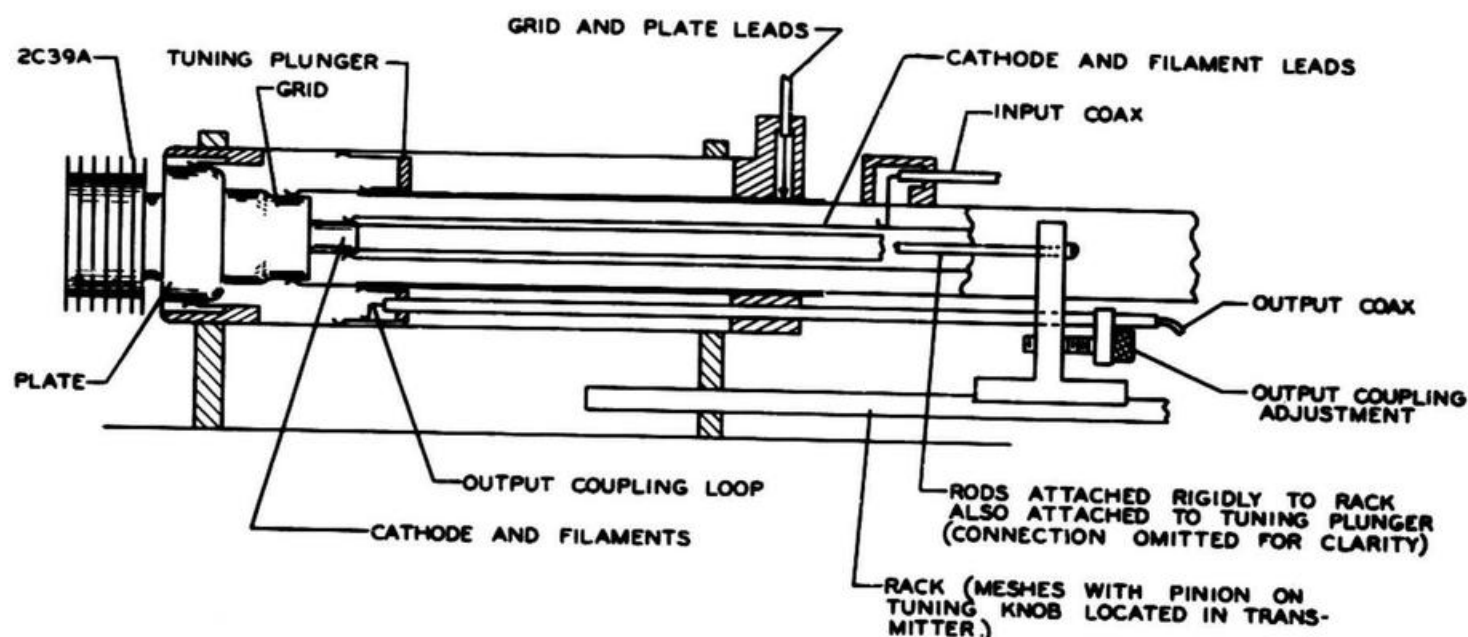
Figure 6-19. Cross Sectional View of Coaxial Resonator
