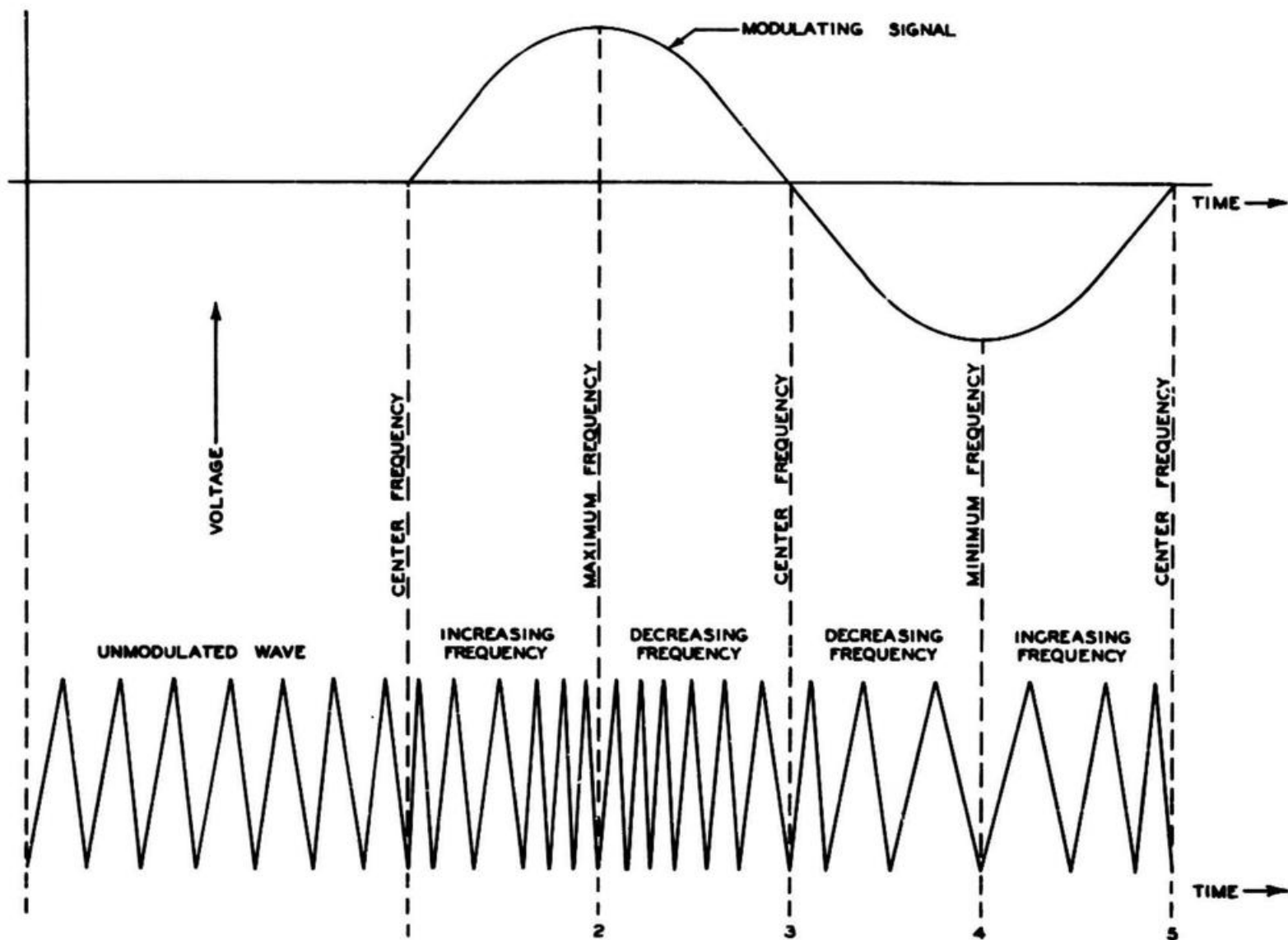
Figure 4-9. Representation of FM
