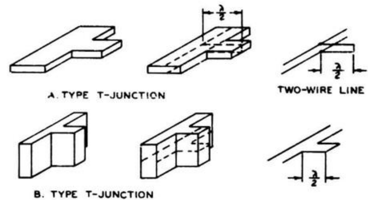
Figure 9-25. T-Junctions
