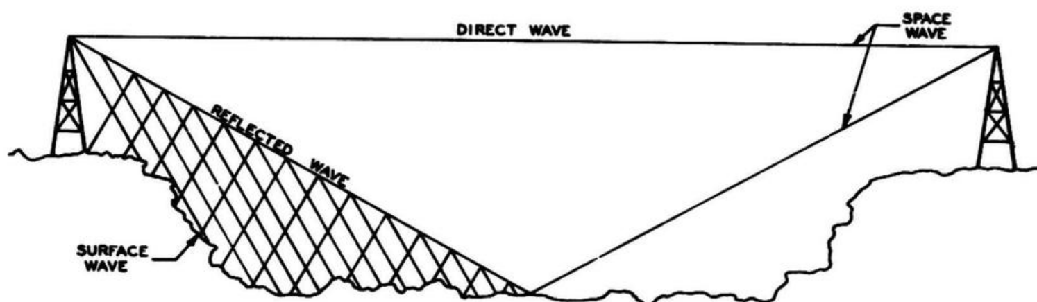
Figure 2-8. Components of the Ground Wave
