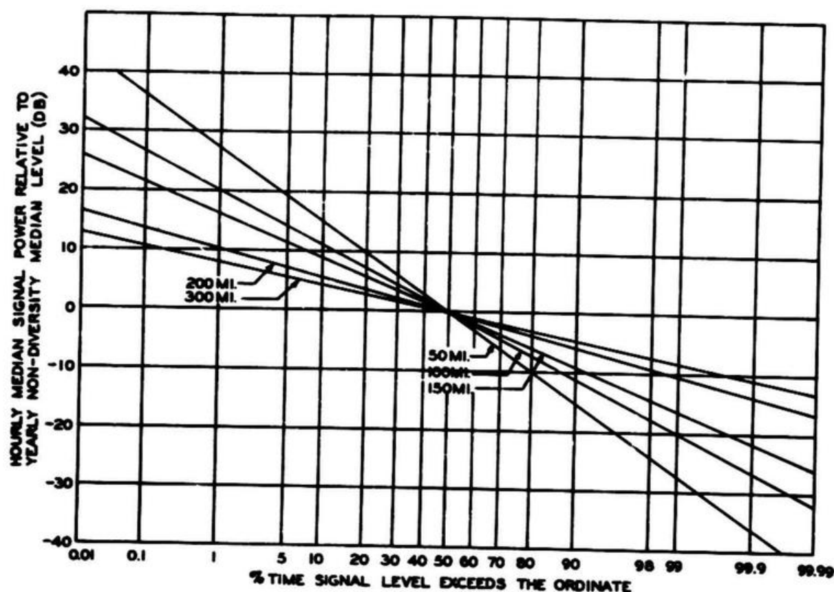
Figure 3-14. Long-Term Distribution of Hourly Medians
