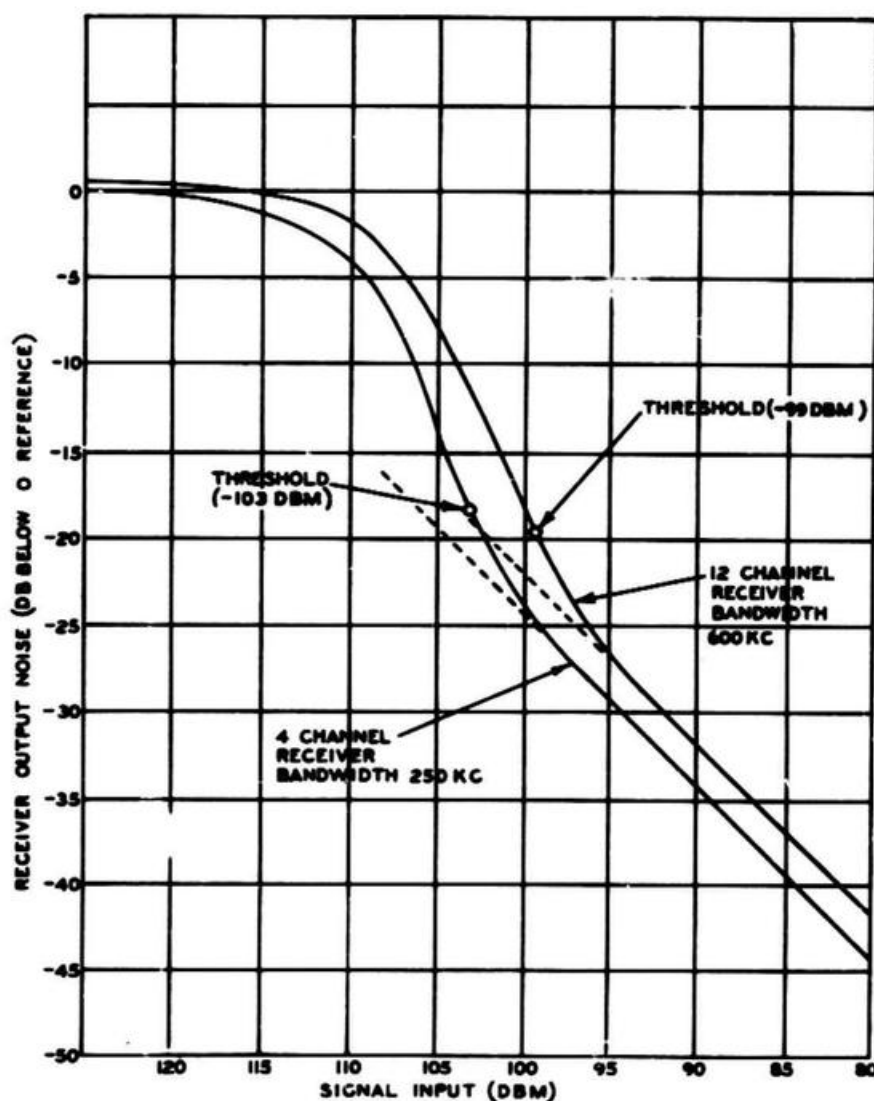
Figure 8-27. Typical Receiver Quieting Curves
