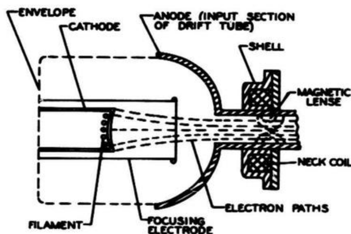
Figure 7-2. Klystron Electron Gun, Simplified Sectional View
