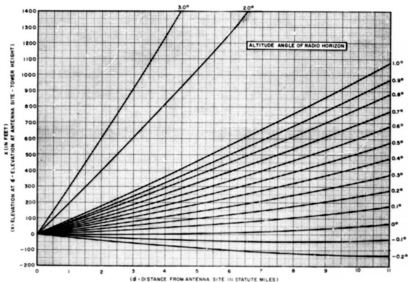
Figure 10-2. Horizon Angle Determination Curves for Short Distances
