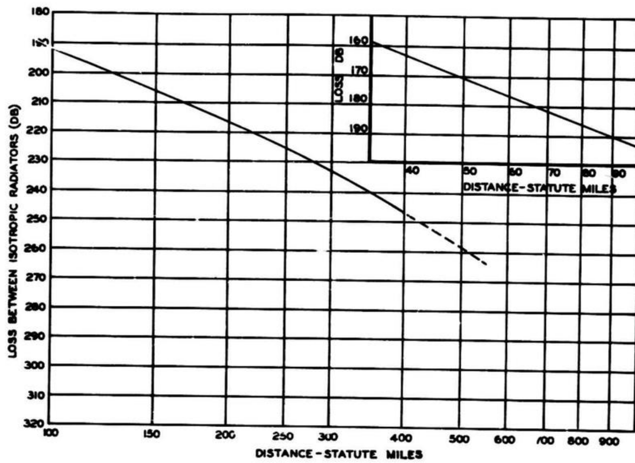
Figure 3-3. Basic Propagation Loss at 1000 Megacycles
