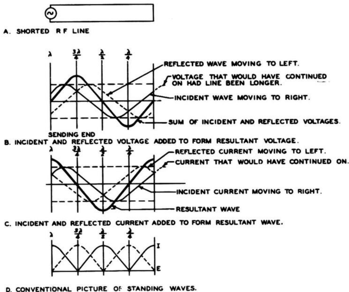
Figure 9-5. Formation of Standing Waves in Shorted Line
