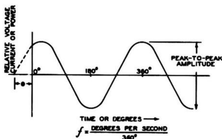
Figure 4-1. Characteristics of the Carrier
