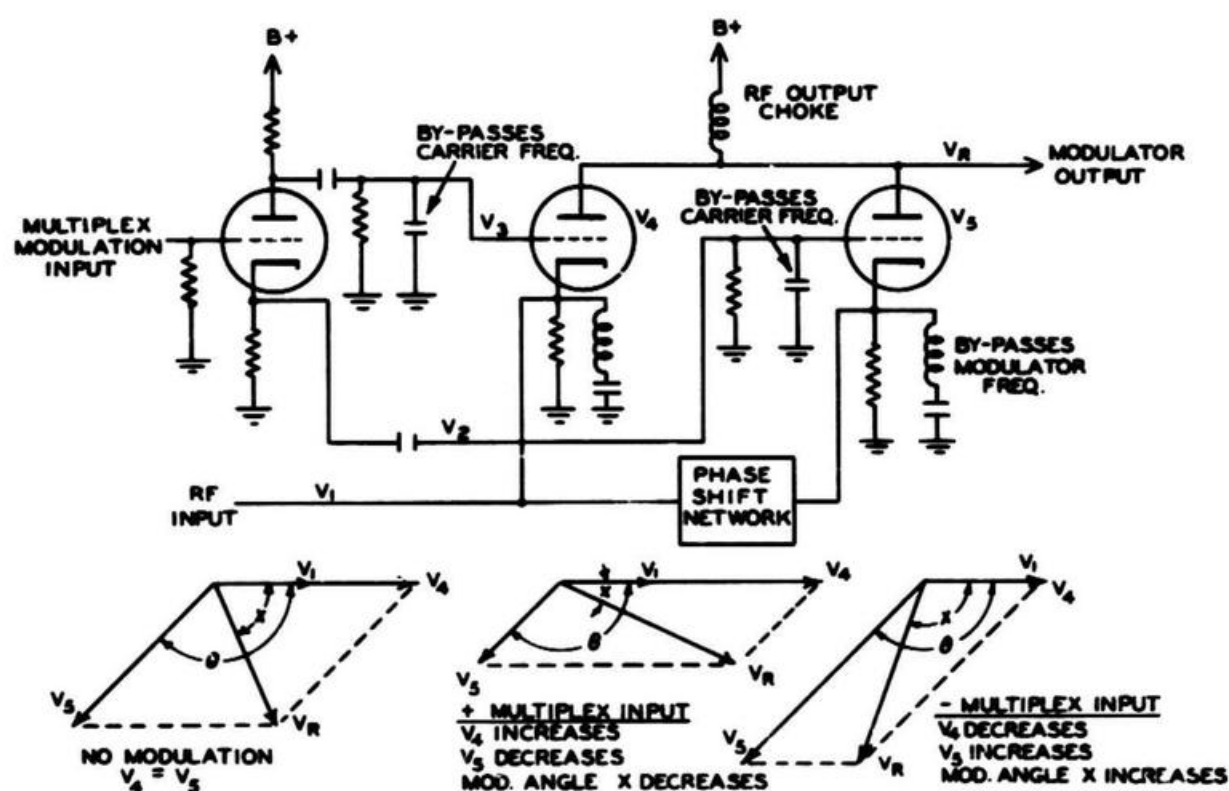
Figure 6-9. Typical Vector Modulator
