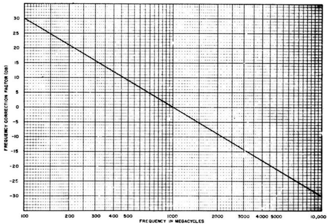
Figure 10-8. Frequency Correction Curve for Basic Propagation Loss
