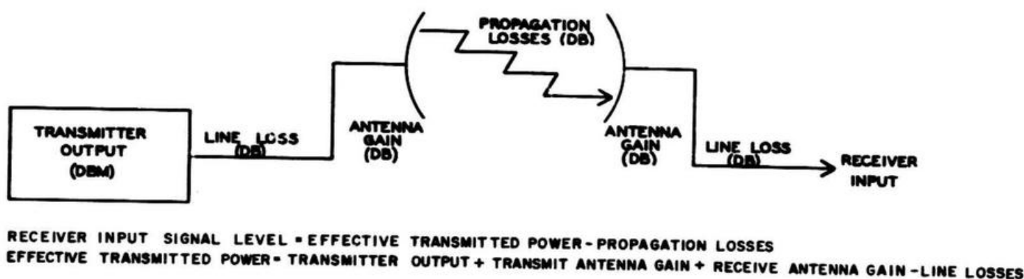
Figure 3-1 Losses and Gains in a Tropospheric Scatter Circuit
