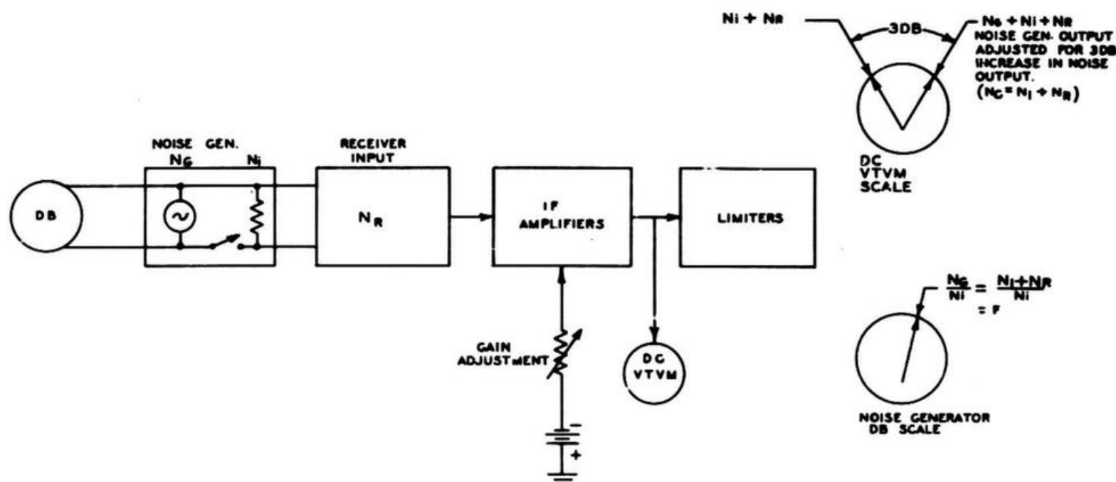
Figure 8-25. Equipment Setup for Determination of Noise Figure
