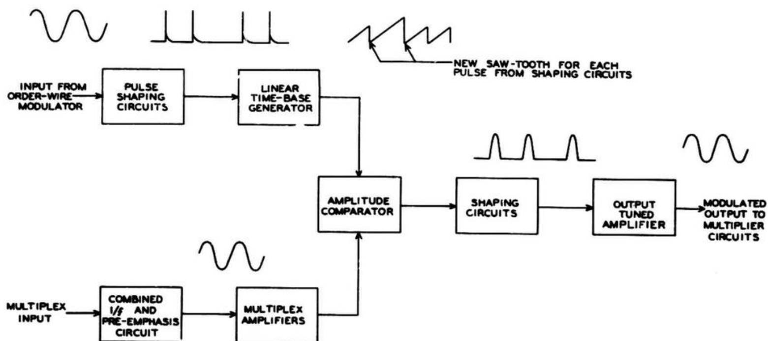
Figure 6-6. Block Diagram of Pulse Phase Modulator
