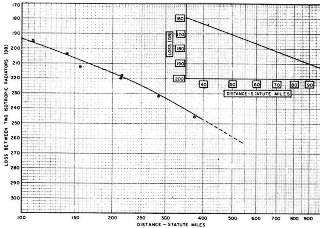
Figure 10-7. Basic Propagation Loss Curve for 1000 Megacycles
